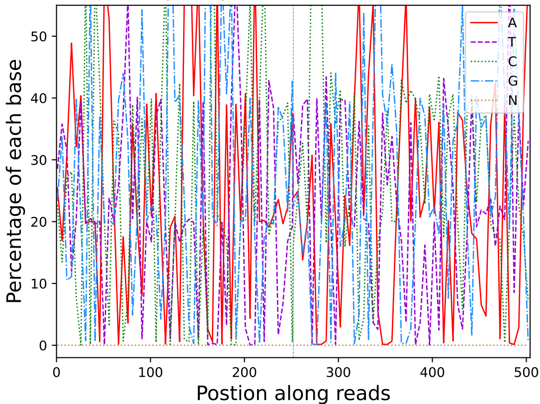
Base percentage along reads (R10306)
